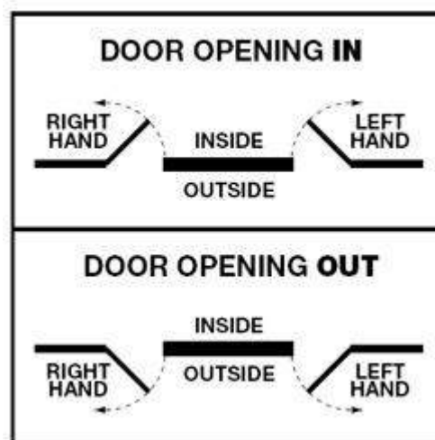
Handing Chart
