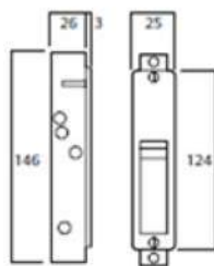
SP3540-SS Security Strike Fabricator Mounting
