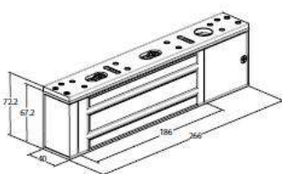
Z8 Electromagnetic Lock
