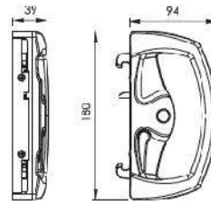
Standard "D" Inner Pull
