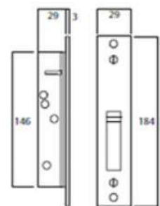
SP3640-SS Security Strike Timber/Metal Jamb
