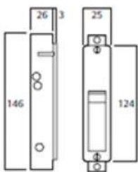
SP3540-LS Latch Strike Fabricator Mounting
