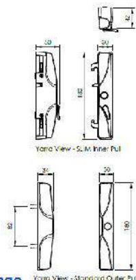
Yarra View - Standard Outer Pull
